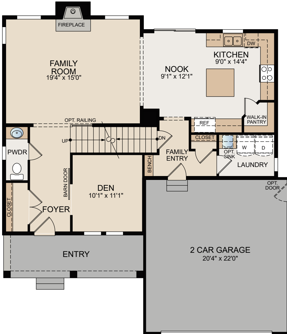
FIRST FLOOR
